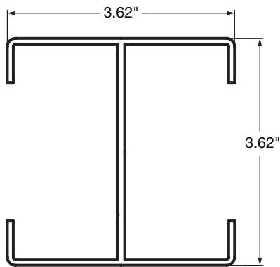
4" Post Stiffener (Redesigned) 018-2 $79.20/24'
