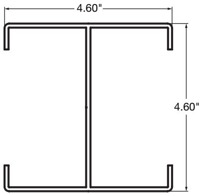
5" Post Stiffener (Redesigned) 018-1 $110.16/24'
