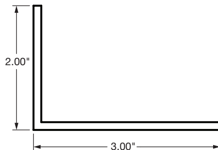
Stiffener Anchor 018-11 $36.00/24'
