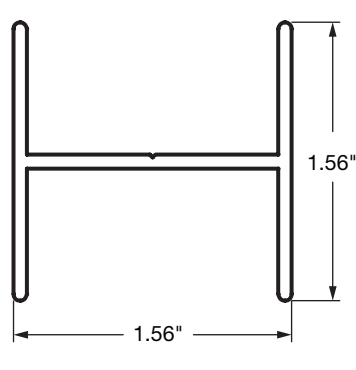
Rail Stiffener 018-5 $20.40/24'
